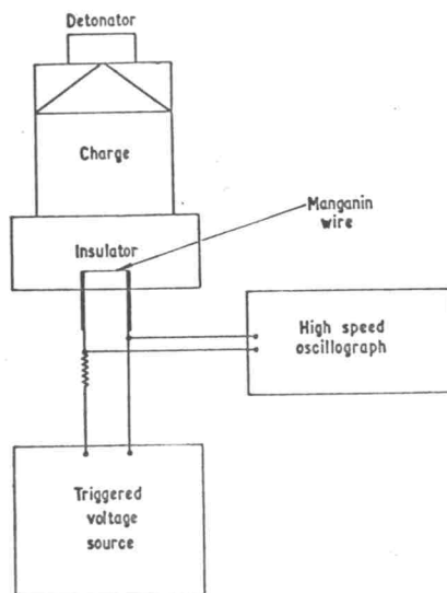
Figure 1. The general arrangement. For simplicity only one wire is shown, but in practice four wires with separate circuits are normally used.
